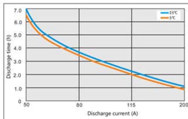
Discharge current VS discharge time curve
