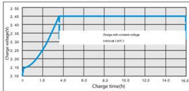
Equalizing charge curve
